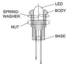
Diffuse
