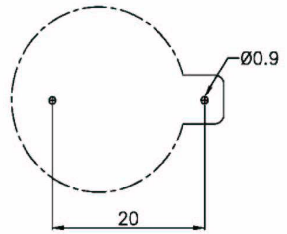
PCB HOLE LAYOUT
